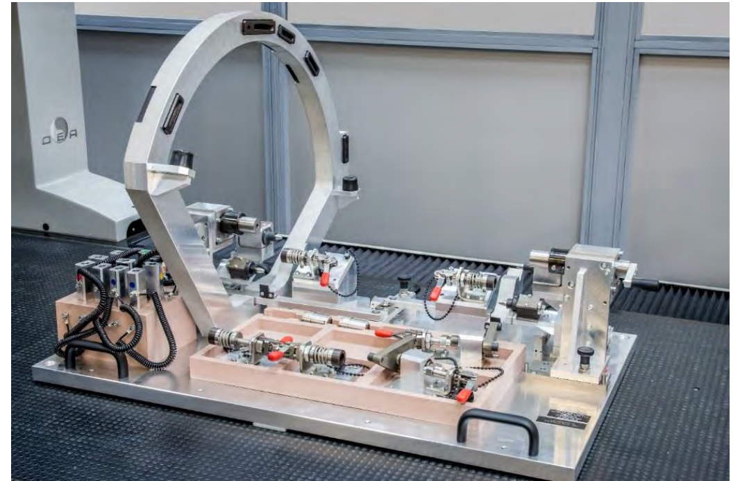
Test stand to control the swing angle of the car seatings
