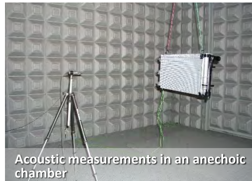
Stand for testing the acoustic properties of materials
