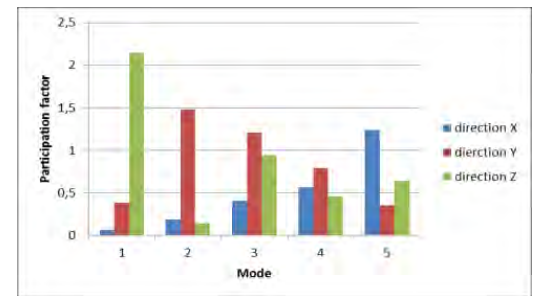
Participation factor for first six modes
